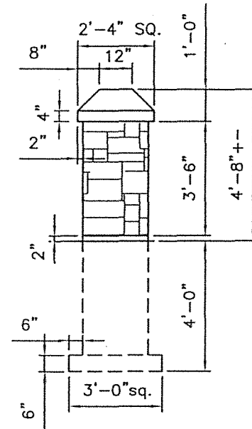
COLUMN DETAIL 1-2 11 INTERMEDIATE COLUMNS REQ'D
