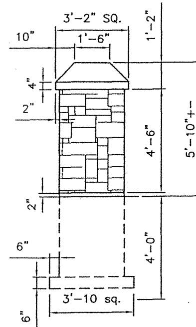
COLUMN DETAIL 2-2 2 END COLUMNS REQ'D
