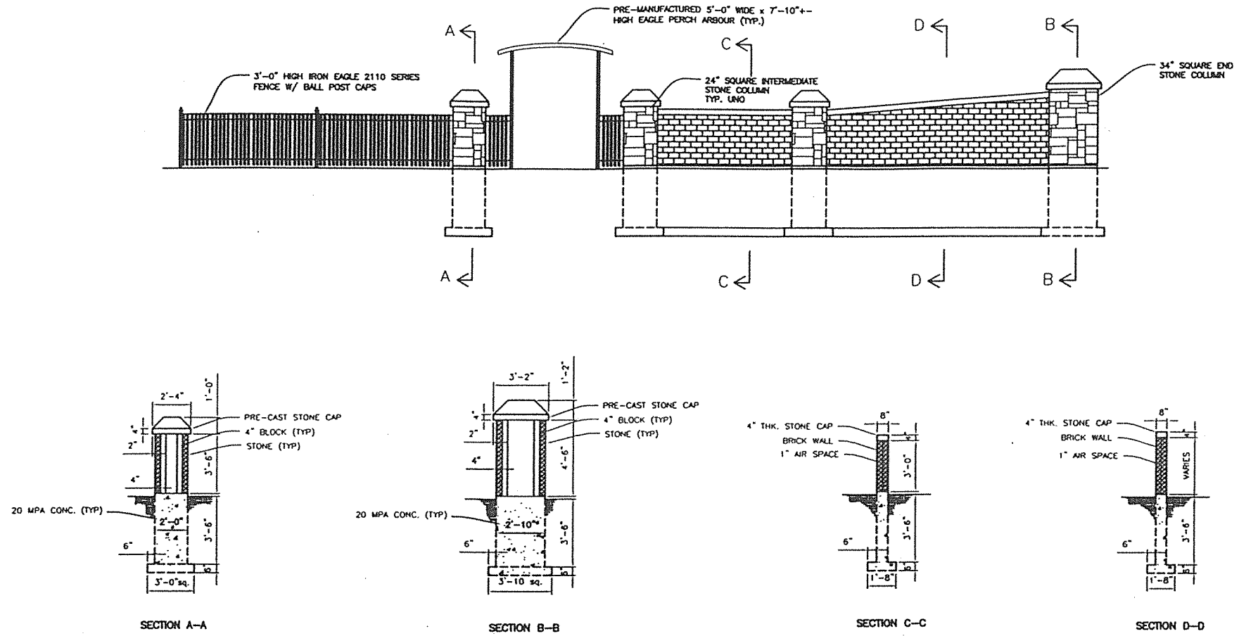
SECTION VIEWS
