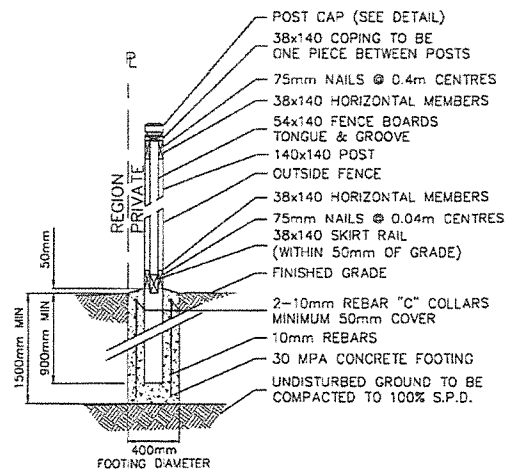
TYPICAL SECTION NTS
