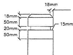
POST CAP DETAIL NTS
