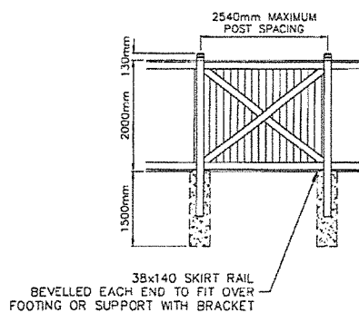
FRONT ELEVATION NTS
